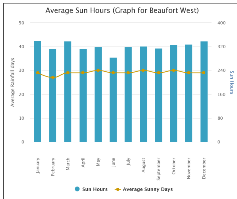
Figure 3.6: The average sun hours and sunny days per month for the Beaufort West area, including the study area for the period 2010 – 2022 (Source: World Weather Online, 2023 6 )
