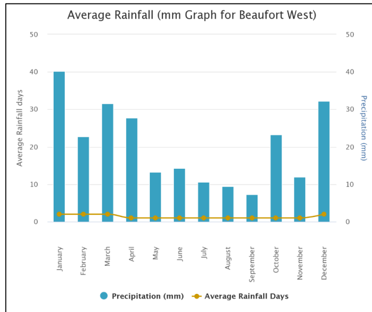
Figure 3.3: The average monthly distribution of rainfall within the Beaufort West area, including the study area (Source: World Weather Online, 2023 3 )
