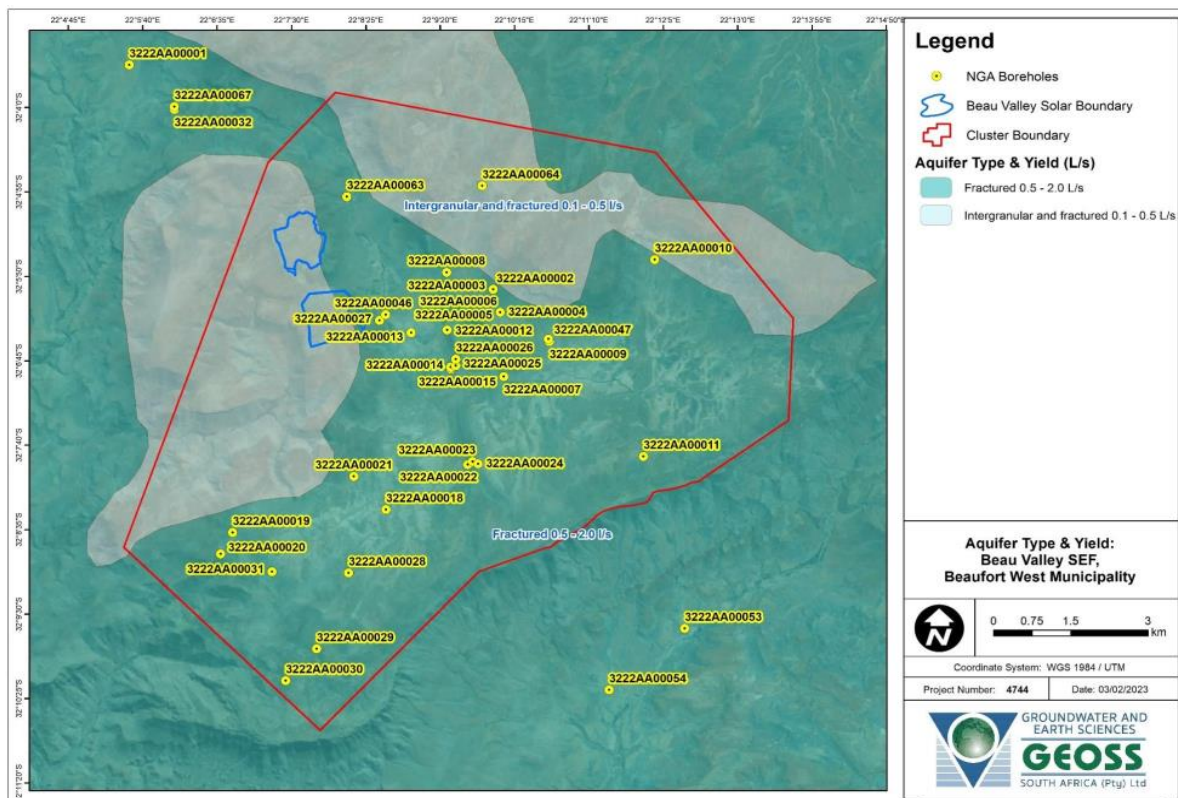
Figure 3.13: Regional aquifer yield and borehole yields (L/s) (Source: DWAF, 2002 and NGA database, in GEOS, 2023, Appendix G.11)
