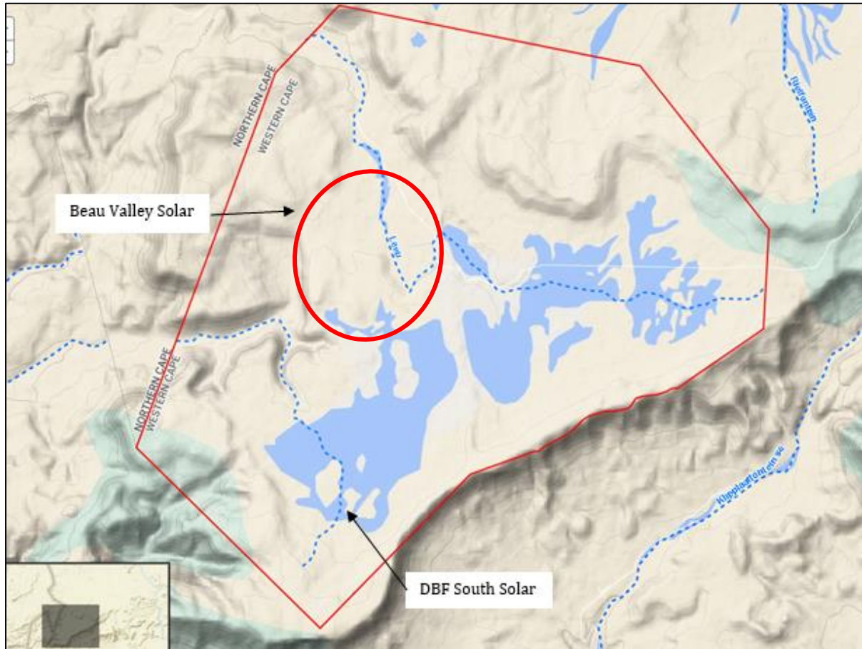
Figure 3.8: Relief map for the area, showing the topography and main watercourses and the location of the projects (CapeFarmMapper, 2023). The red oval shows the focus area for the proposed project.
