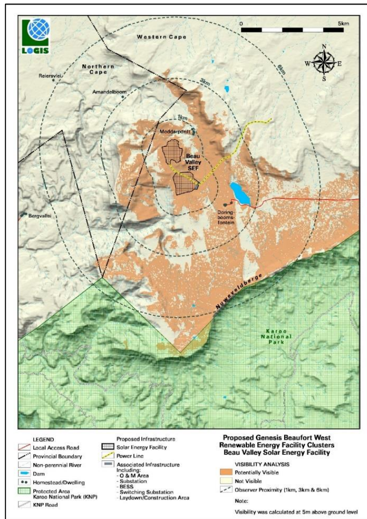
Figure 3.32: Potential visual exposure (visibility analysis) for Beau Valley SEF shown in relation to the northern edge of the Karoo National Park (green-shaded area). (Source: Appendix G.5).
