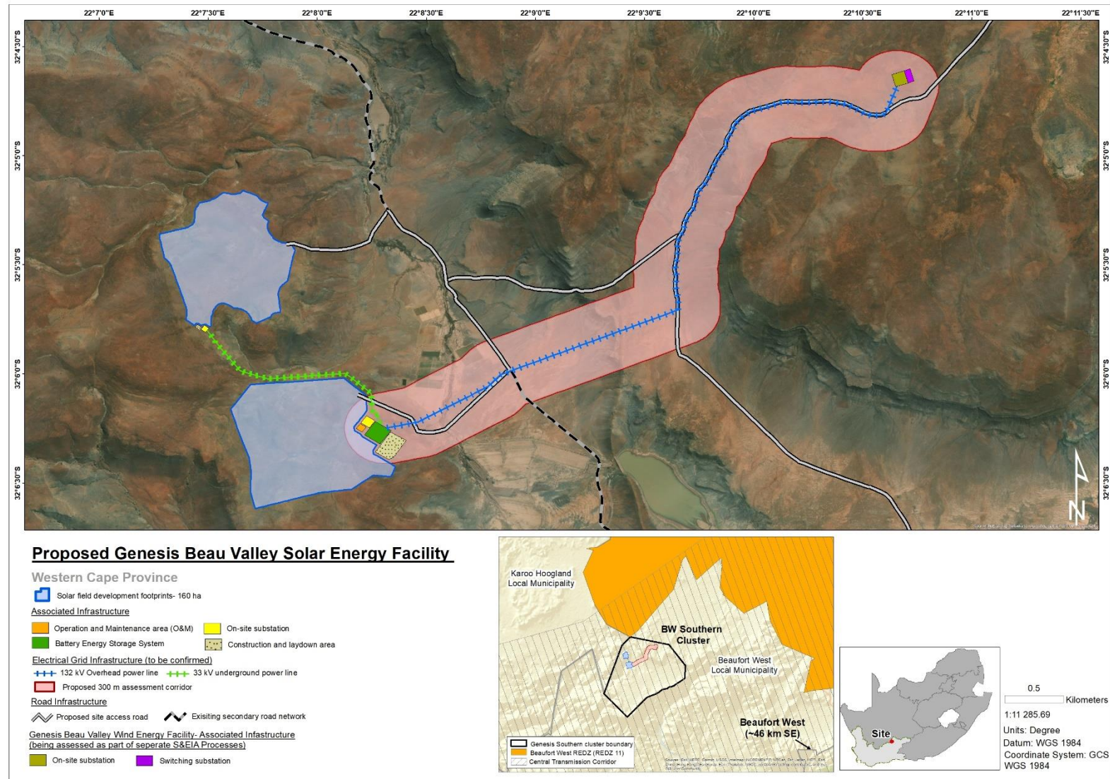
Figure 7.1: Site layout recommended by the EAP for approval for the proposed Beau Valley SEF project which was assessed during the EIA Phase.
