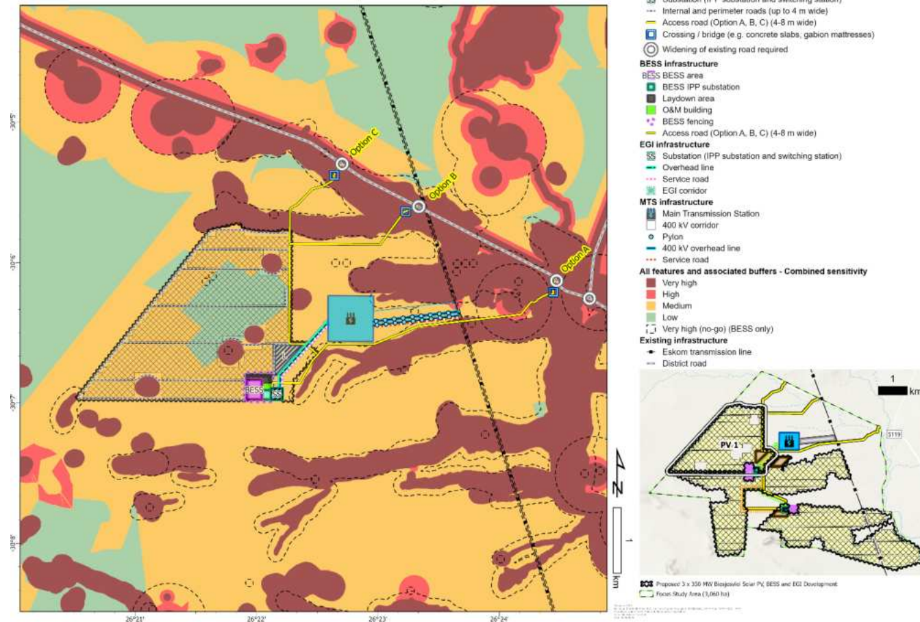
Figure 20.8: Combined Final Project Layout and Sensitivity Map for Project 1 (Biesjesvlei PV1), Project 4 (Biesjesvlei BESS 1), and Project 7 (Biesjesvlei EGI 1) [including Project 10 (Biesjesvlei MTS and LILO)].
