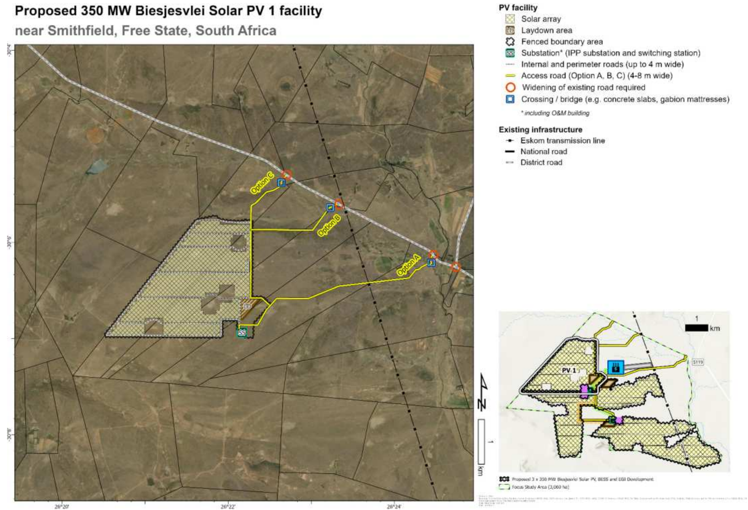
Figure 20.1: Final Project Layout Map showing the detailed infrastructure and development footprints for Biesjesvlei PV1.
