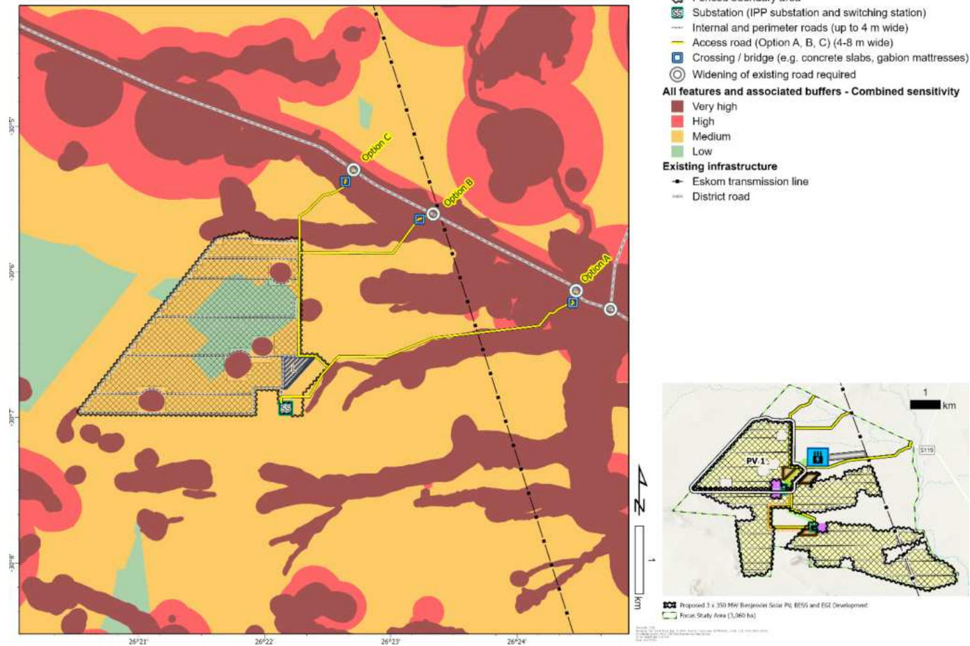
Figure 20.5: Combined Final Project Layout and Sensitivity Map for Biesjesvlei PV1.
