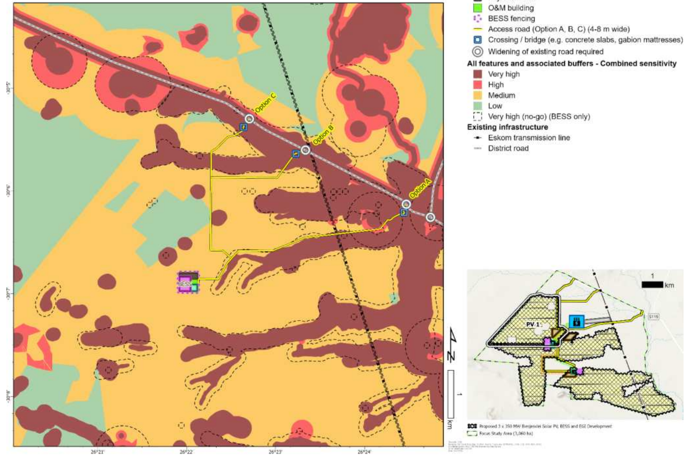
Figure 20.6: Combined Final Project Layout and Sensitivity Map for Biesjesvlei BESS 1.
