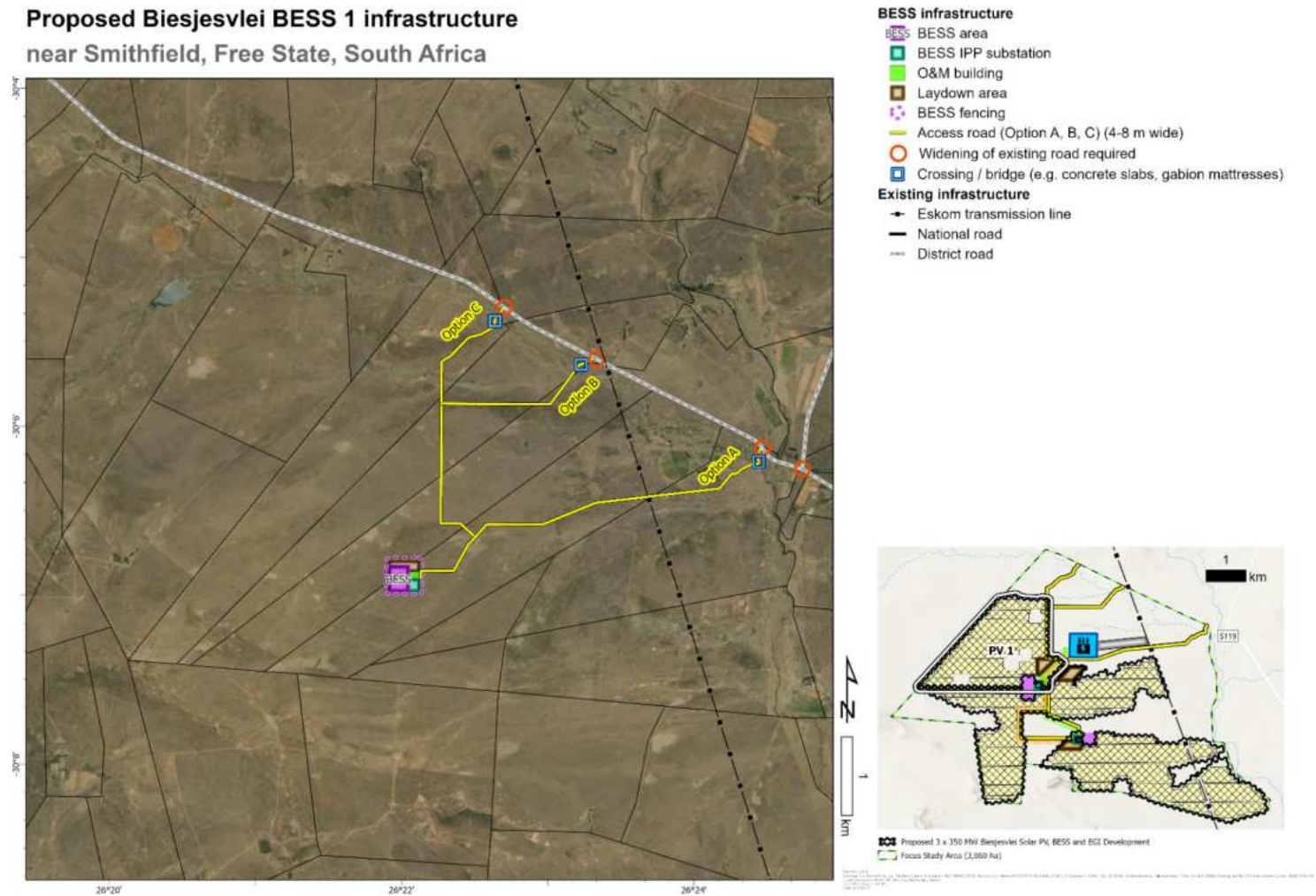
Figure 20.2: Final Project Layout Map showing the detailed infrastructure and development footprints for Biesjesvlei BESS 1.
