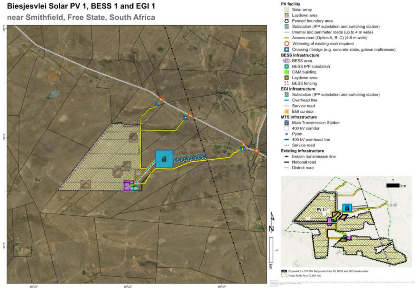
Figure 20.4: Final Project Layout for Project 1 (Biesjesvlei PV1), Project 4 (Biesjesvlei BESS 1), and Project 7 (Biesjesvlei EGI 1) [including Project 10 (Biesjesvlei MTS and LIL0)].
